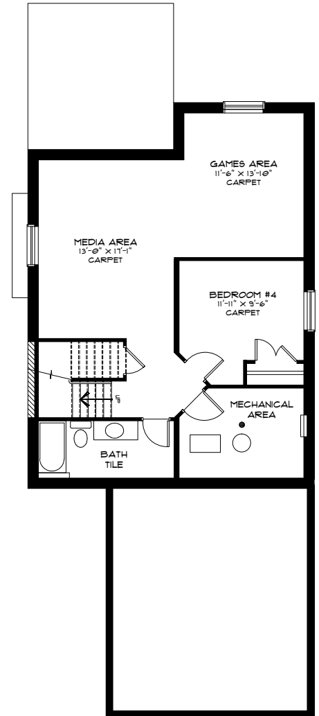
Optional Lower Floor 700 Sq. Ft.
