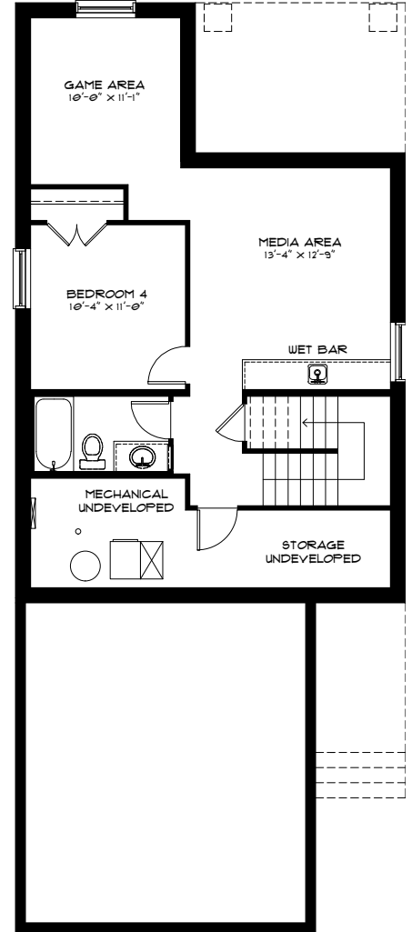
Optional Lower Floor 620 Sq. Ft.
