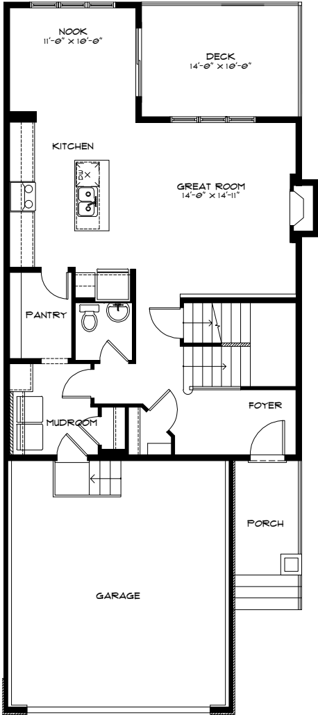
Main Floor 900 Sq. Ft.
